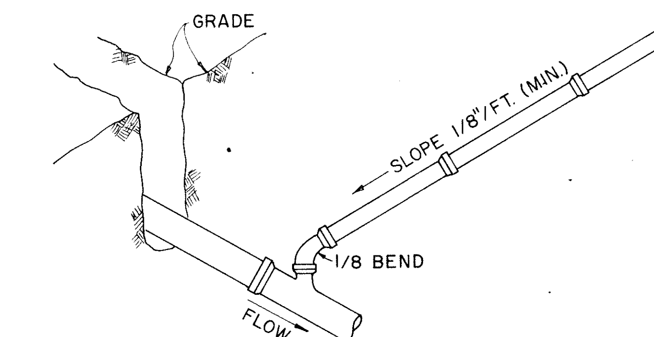
SANITARY SEWER CONNECTION
