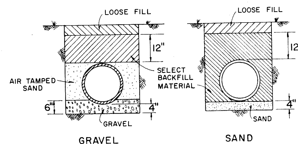
PIPE BEDDING AND EMBEDMENT
