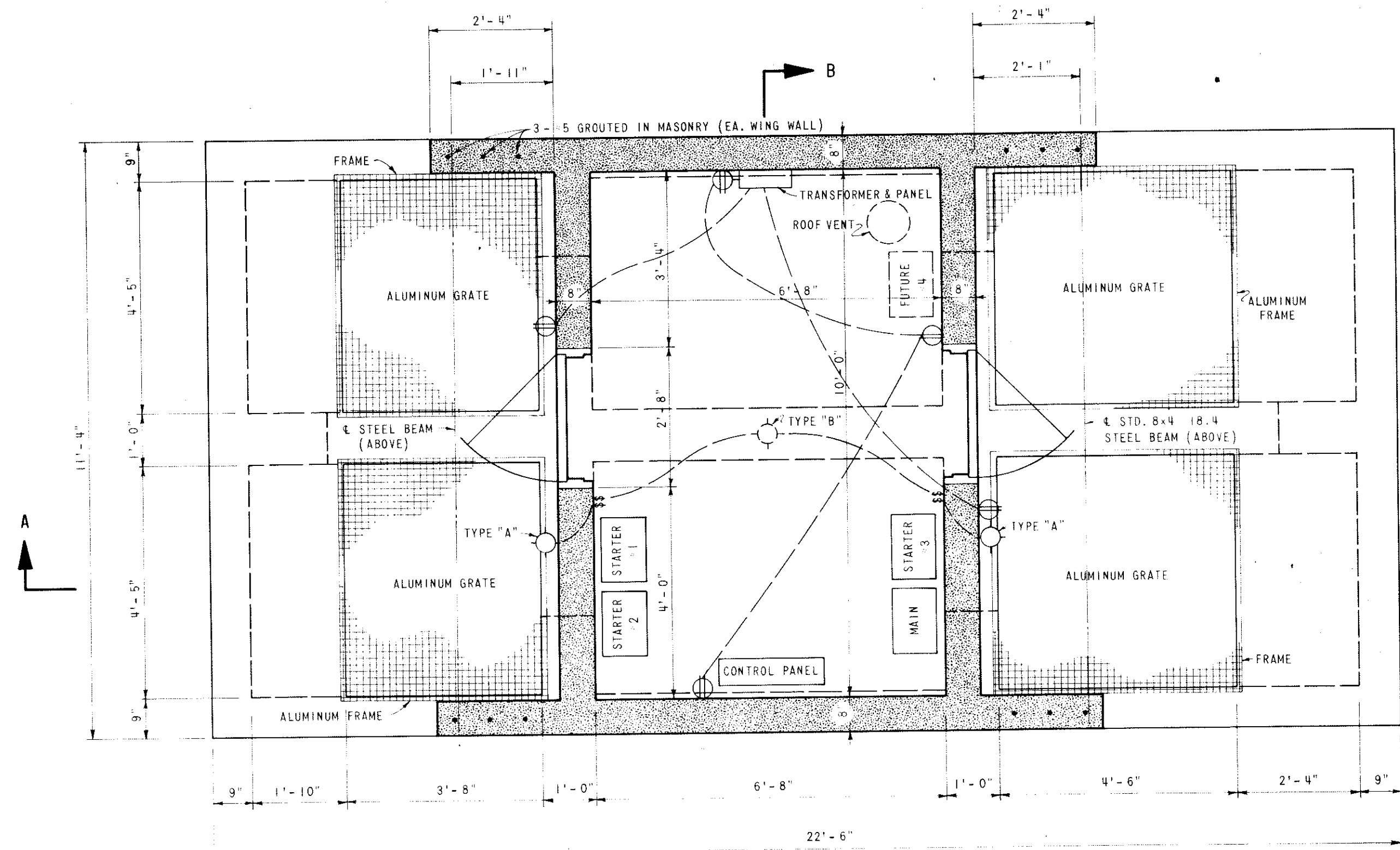
UPPER PLAN
