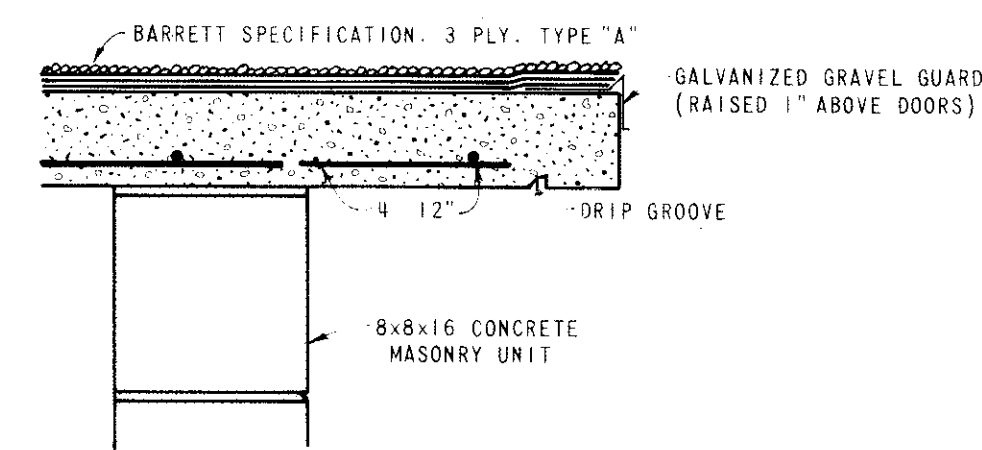
ROOFING DETAIL SCALE: 1 1/2" = 1'-0"
