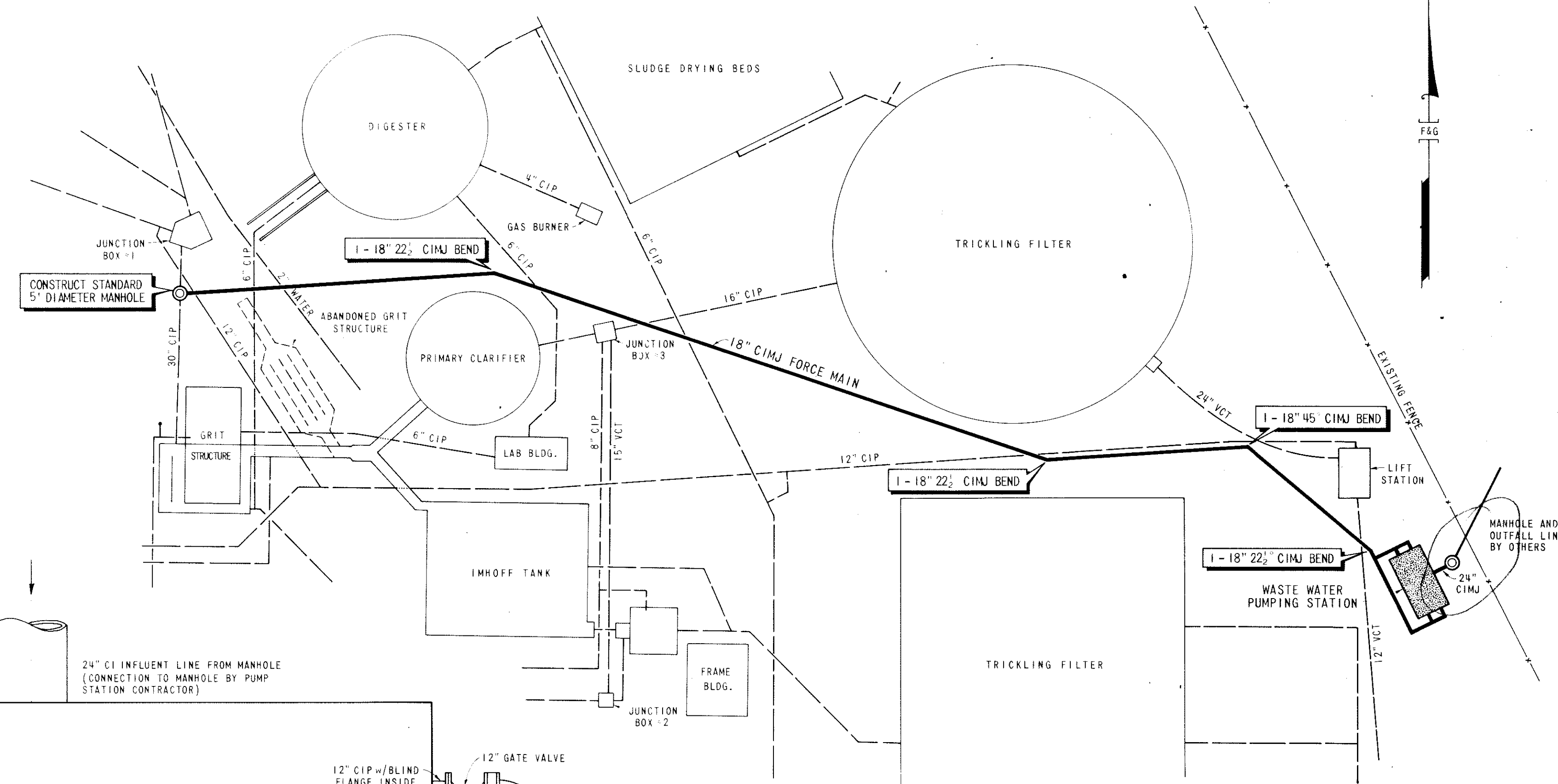
SITE PLAN SCALE: 1" = 30'
