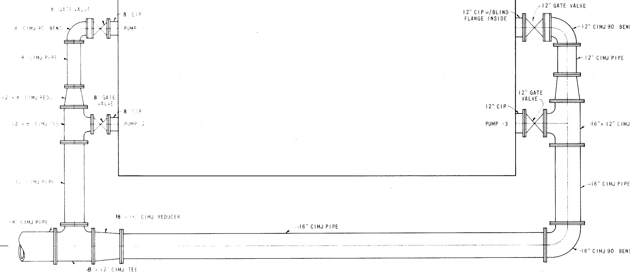
EXTERIOR PIPING LAYOUT SCALE: 1/2" = 1'-0"
