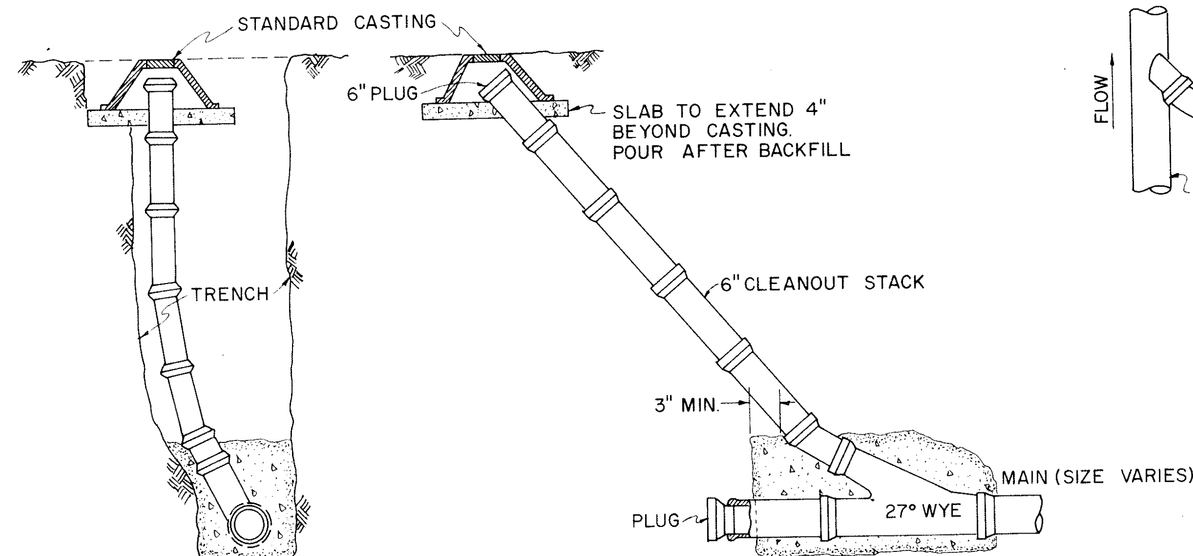
SANITARY SEWER CLEANOUT
