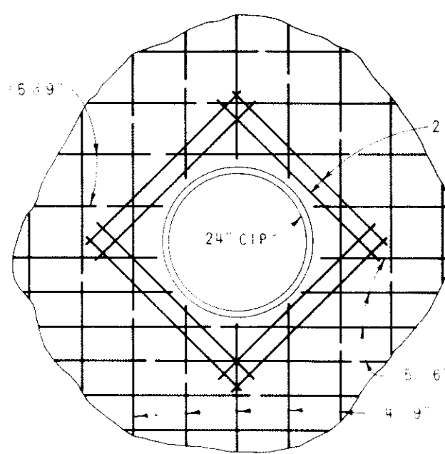
DETAIL AT 24" CIP OPENING SCALE: 1/2" = 1'-0"
