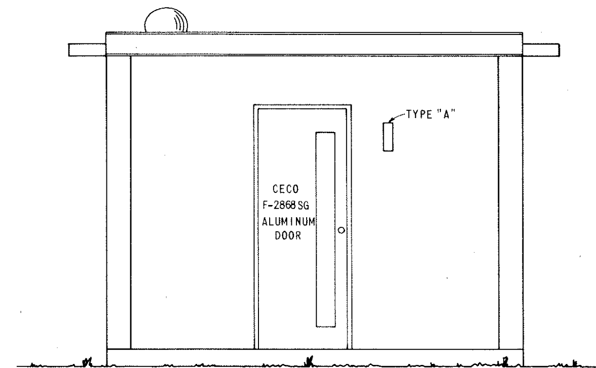
NORTH ELEVATION SCALE: 1/2" = 1'-0"
