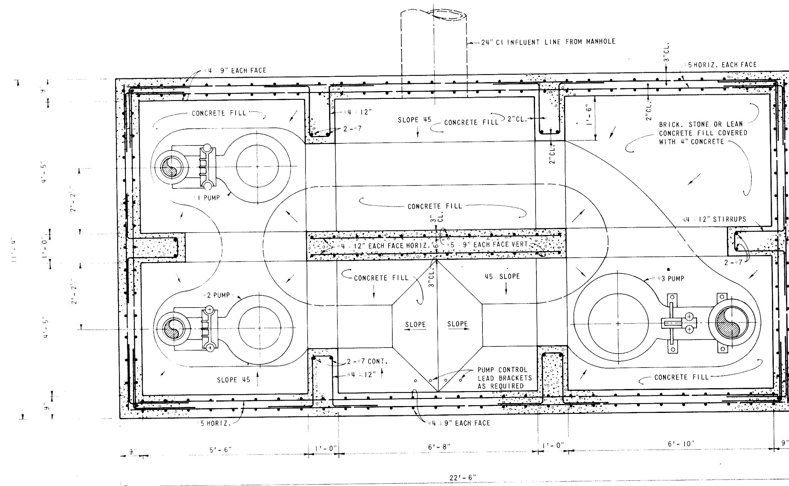
LOWER PLAN - SECTION C-C SCALE: 1/2" = 1'-0"
