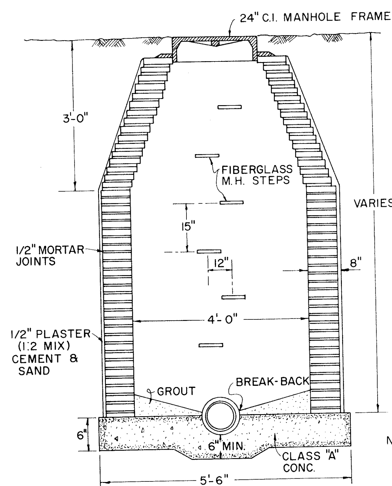
MANHOLE DETAIL NO SCALE
